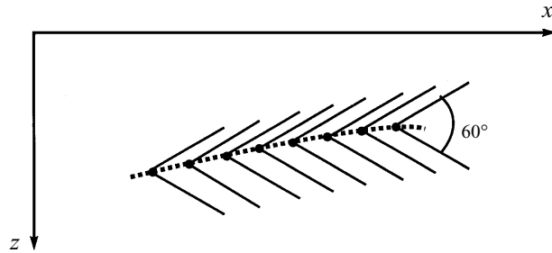
FIGURE 5. Schematic for the detection of the quasi-streamwise structure. The dots represent the locations of local maximum of -\lambda_2 and the solid lines denote cones at \pm 30^\circ ; the thick dashed line represents the vortex axis.
