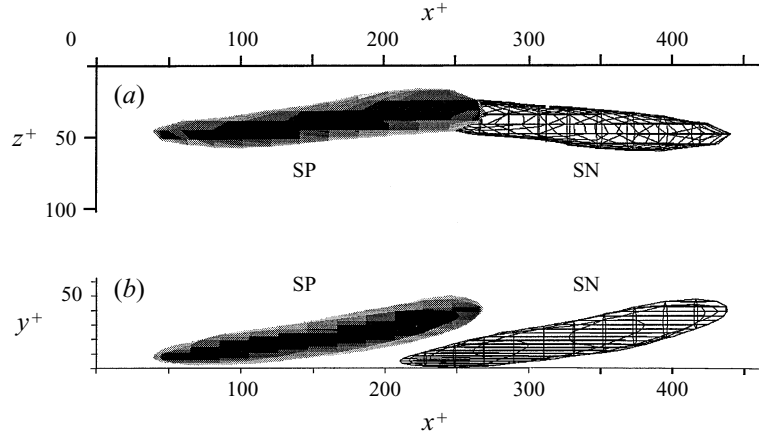
FIGURE 6. Contour plot for \lambda_2(\partial\langle u_i\rangle/\partial x_j) of SP and SN in (a) top view; (b) side view. The shaded and wire frame surfaces represent SP and SN respectively. These structures are superimposed to show their relative locations and orientations.
